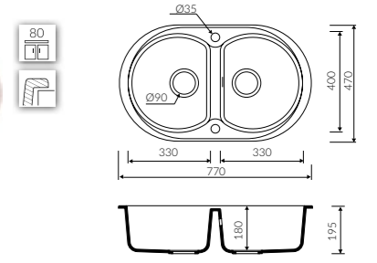
DURO 770 2K Index: P_Z_025_20_0770 L 770 W 470 H 195 mm
