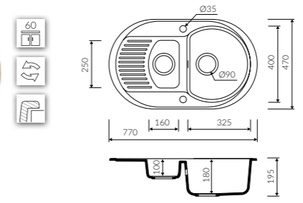
DURO 770 1,5KO Index: P_Z_025_51_0770 L 770 W 470 H 195 mm
