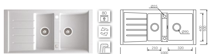
PROFIR 1000 1,5KO Index: 160 513 0xx L 1000 W 500 H 230 mm
